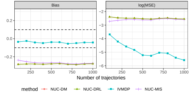
Figure 4. Bias (left panel) and logarithmic MSE (right panel) and as the sample size increases. The two dashed lines correspond to the Monte Carlo error bounds for the bias. As we can see from the figure, only our approach is empirically unbiased and achieves the smallest MSE.
