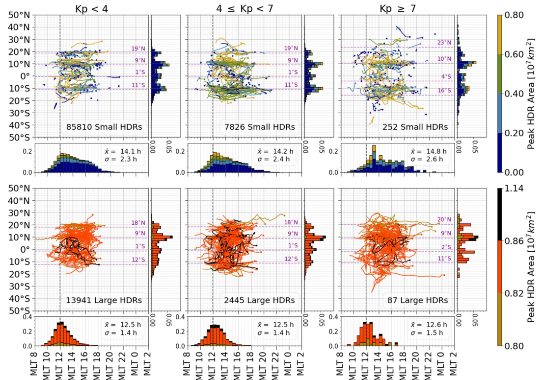
Figure 6. HDR trajectories plotted in SM coordinates. Each panel plots HDR paths for each label at different levels of Kp. The top row plots small HDRs and the bottom row plots large HDRs. Each column shows HDRs that occur during different activity levels, labeled at the top. Path endings are indicated by a filled circle. For K_p < 7 line plots are a sample equal to the number of HDRs in the extreme case. Paths are colored based on peak HDR area for that duration, with color-bars provided on each row. MLT 12 is marked with a black dashed vertical line for each panel. Horizontal purple dashed lines at constant latitude mark K-means centroids for each of the four clusters found, labeled with the calculated magnetic latitude value. PDFs for the location at which HDRs form in MLT and magnetic latitude are plotted alongside each panel along the relevant axes. They are colored based on the peak HDR area. The histograms are normalized to integrate to 1. The sample mean \bar{x} and standard deviations \sigma for MLT distributions are given in legend of these panels in hours.
