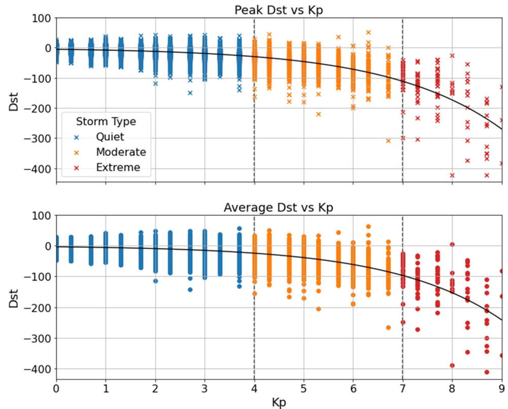
Figure C1. Peak/average hourly Dst over a 3-hr interval versus Kp. The plot is split between the three different storm conditions defined in Section 4.2: quiet ( K_p < 4 ), moderate ( 4 \leq K_p < 7 ) and extreme ( K_p \geq 7 ). The bounds are indicated by vertical dashed lines and each storm type is color-coded as per the legend in the top panel. A fitted exponential curve is plotted in black.
