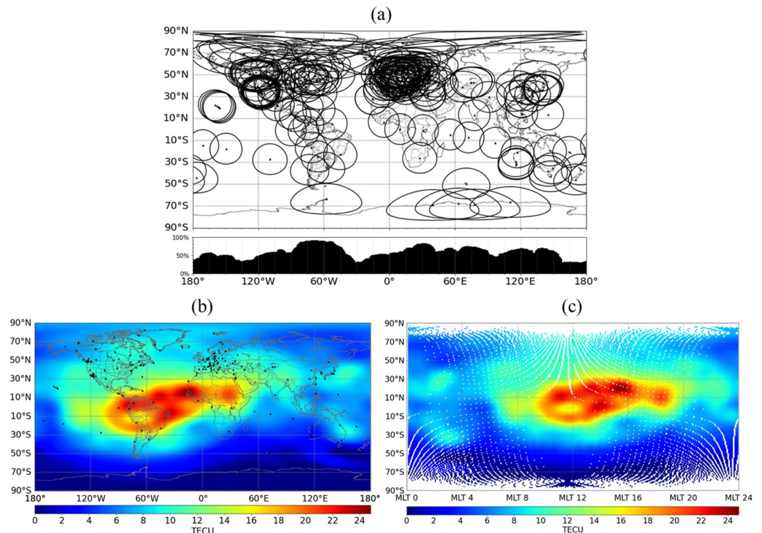
Figure 1. Example TEC map for 2009 – 07 – 23 at 16 : 30 : 00 UTC in geographic coordinates. Panel (a) plots ground stations that provide the data compiled on this date, black lines plot great circles at 10^\circ inclination to indicate the coverage of each station. A histogram of the percentage of grid points at every 1^\circ of longitude enclosed by these great circles is plotted across the bottom of panel (a). Panel (b) plots the resulting geographic TEC map for this date-time. Each 1^\circ \times 1^\circ grid point plots the VTEC at that longitude/latitude. Black triangles show the locations of ground stations in both sub-figures. Panel (c) plots the same TEC map in Solar Magnetic (SM) coordinates (geomagnetic latitude vs. MLT). White grid points in the map are regions of undefined TEC resulting from the coordinate transform. The TEC values are indicated by the color-bar at the bottom of each TEC map.
