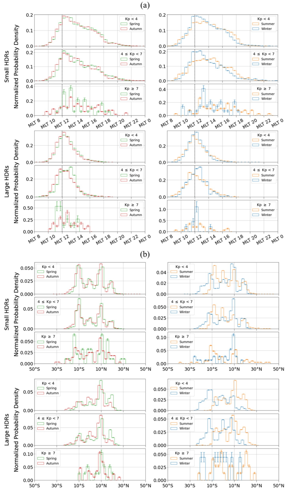
Figure 7. Seasonal histograms for the coordinates where HDRs first form. Sub-figure (a) plots MLT and sub-figure (b) plots the magnetic latitude. MLT 12 is marked as dashed lines in each panel of (a). The top group of each sub-figure plots small HDRs and the bottom group plots large HDRs. Each row plots data within a given Kp range, denoted in the legend. Spring/autumn are plotted on the left-hand column and summer/winter are plotted on the right-hand column. Error bars due to the sample size are plotted.
