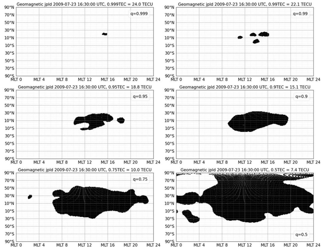
Figure B1. Isolated HDRs for the TEC map on 2009 – 07 – 23 at 16 : 30 : 00 UTC in geomagnetic coordinates using different quantile thresholds: q = 0.999, 0.99, 0.95, 0.90, 0.75 and 0.50 . The value of TEC for these quantile thresholds is given in the title of each plot, along with the date and map type.
