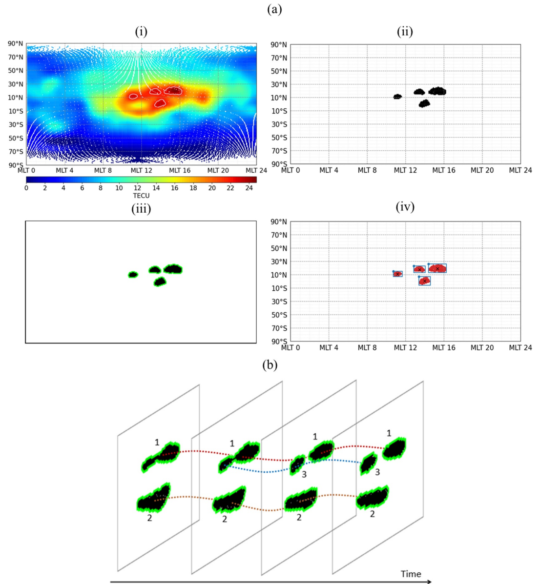
Figure 4. Sub-figure (a) outlines the procedure for HDR identification and tracking shown for TEC maps for 2009 – 07 – 23 at 16 : 30 : 00 UTC in geomagnetic coordinates. Panel (i) plots the geomagnetic TEC map with gray contours at the top 1% value of TEC in the map, defining the High Density Regions (HDR). Panel (ii) isolates these HDRs and plots them in black. Panel (iii) shows the binary image of the HDRs with green contours drawn around each black region to demonstrate the algorithm's contour detection. Panel (iv) plots the isolated HDRs in SM coordinates with bounding rectangles in blue and centroids marked in black, obtained by the detection/tracking algorithm. Sub-figure (b) demonstrates the labeling process for consecutive images for the date 2013 – 04 – 02 from 09 : 30 : 00 to 10 : 15 : 00 UTC. Dashed lines connect the same labeled HDRs between images, with different colors for each unique HDR.
