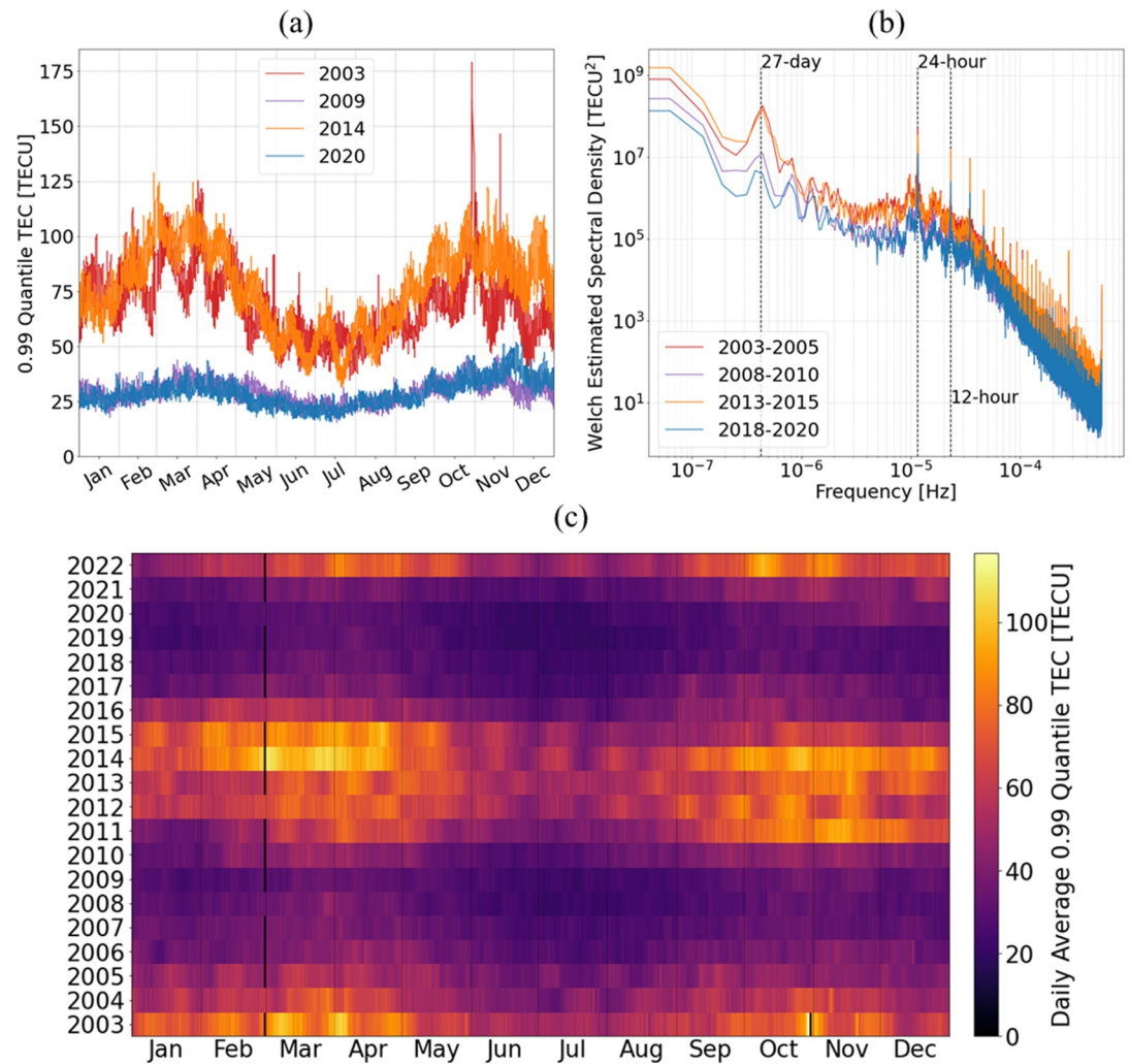
Figure 3. TEC climate as seen in the long-term variation of the 0.99 quantile of TEC. Panel (a) plots year-long time-series for 2 years during solar maximum (2003 and 2014) and 2 years during solar minimum (2009 and 2020). Panel (b) plots the Welch-estimated power spectrum for 3-year long intervals during solar maximum (2003 – 2005 and 2013 – 2015) and solar minimum (2008 – 2010 and 2018 – 2020). Vertical black dashed lines indicate frequencies at 12-hr, 24-hr, and 27 days. Panel (c) plots the daily averaged 0.99 quantile TEC on a year versus month grid. Black grid points indicate no data for that day, or alignment with leap days.
