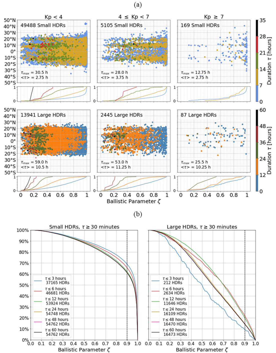
Figure 9. Sub-figure (a) plots the magnetic latitude of HDR formation plotted against the ballistic parameter \zeta . The top row plots results for small HDRs and the bottom row for large HDRs. Each point is colored by the duration \tau of the HDR, color-bars provided on each row, and the smallest durations are plotted underneath the longest durations. The number of HDRs and the maximum/average durations are shown in each axis. Below each axis the CDFs are plotted for \zeta colored based on the duration bands defined by the color bar. Only HDRs with durations \tau \geq 30 minutes are plotted. Sub-figure (b) plots the percentage of HDRs that exceed a given value of \zeta for small (left panel) and large (right panel) HDRs with durations \tau \leq 3, 6, 12, 24, 48 and 60 hr. The number of HDRs within each data sub-set is shown in the legend for each axis. Vertical dashed lines indicate the choice in \zeta above which an HDR is defined to follow a ballistic trajectory.
