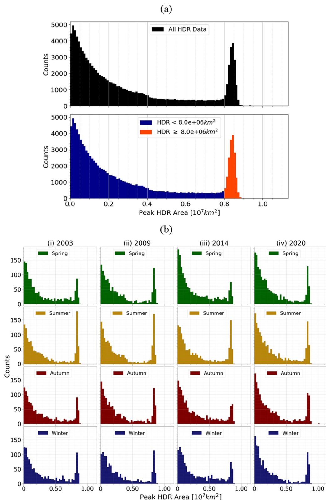
Figure 5. Sub-figure (a) plots distributions of the maximum area for each unique HDR in the data -set. The upper panel plots all the data and the bottom plots the distribution split into large (orange) and small (blue) HDRs, separated by an area of 8 \times 10^6 \text{ km}^2 . Sub-figure (b) plots these area distributions divided by for calendar years (i) 2003, (ii) 2009, (iii) 2014 and (iv) 2020. Histograms are normalized to integrate to 1.
