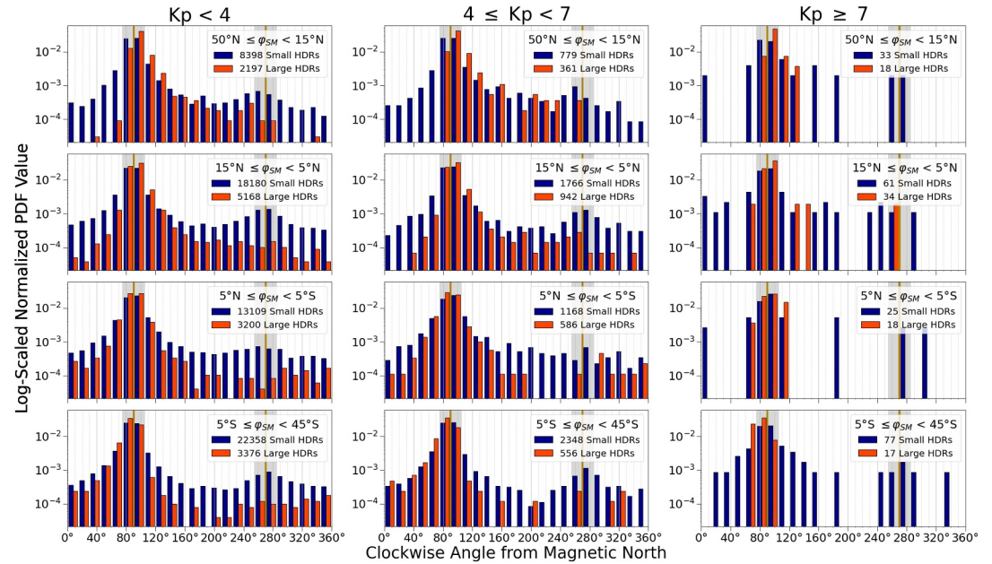
Figure 8. Log-scaled histogram plots of the magnetic bearing \beta , the clockwise angle from magnetic north, for large (orange) and small (blue) HDRs in 15^\circ bins. The histograms are normalized to integrate to 1. Each panel plots net trajectory bearings within a latitude band for each K-means cluster determined in Figure 6 for different activity levels shown in each column. Legends in each panel indicate the latitude band and the number of small/large HDRs that form in these regions. The shaded regions \pm 15^\circ from \beta = 90^\circ and \beta = 270^\circ indicate motion with approximately constant magnetic latitude. Only HDRs with durations \tau \geq 15 minutes are included.
