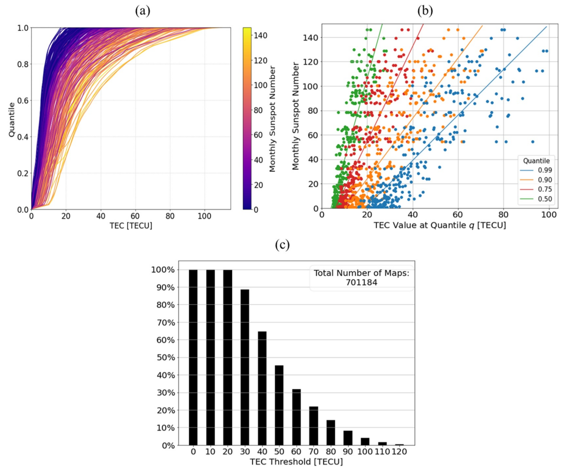
Figure 2. Panel (a) plots the CDFs of a subset of maps from solar cycle 24 (between 2009 and 2020) at 12 : 00 : 00 UTC. Each line is color-coded to indicate the monthly mean sunspot number for that date-time. Panel (b) plots the monthly mean sunspot number for the same subset of maps against the associated TEC value for the given quantiles q = 0.99, 0.9, 0.75 and 0.5 , defined in the legend. A straight line is fitted to each quantile data group. Panel (c) plots the percentage of maps which have a maximum TEC value that exceeds a given TEC threshold, obtained for 20 years of 15 min maps.
